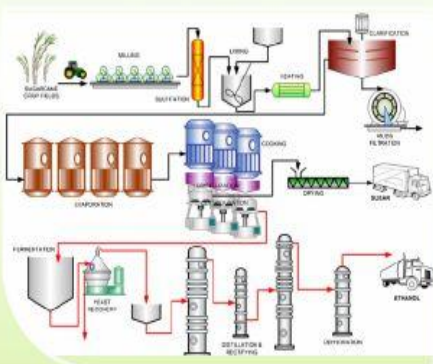
Bio-ethanol Extraction Process through Sugarcane
